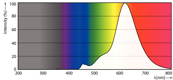
Spectral Power Distribution Colour - MAS VLE LEDLusterD 2.6-15W E14 P45 SP G
